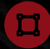
UI/UX Design
